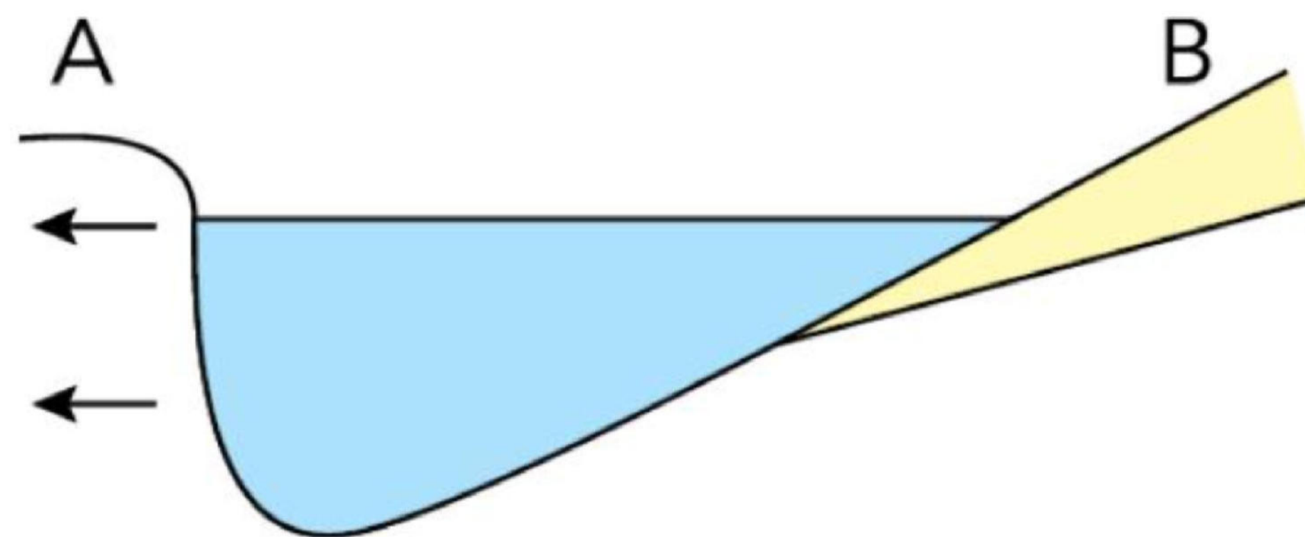
Figure 1.3: A cross-section through a meander bend in a river
